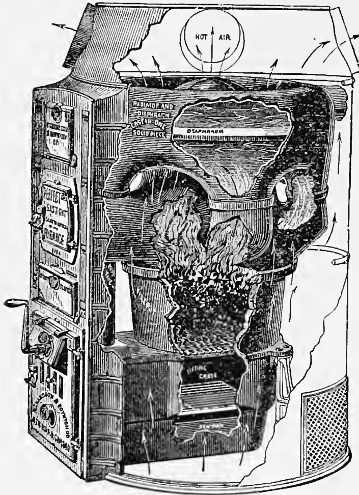
PERFECT Warm Air Furnace.
